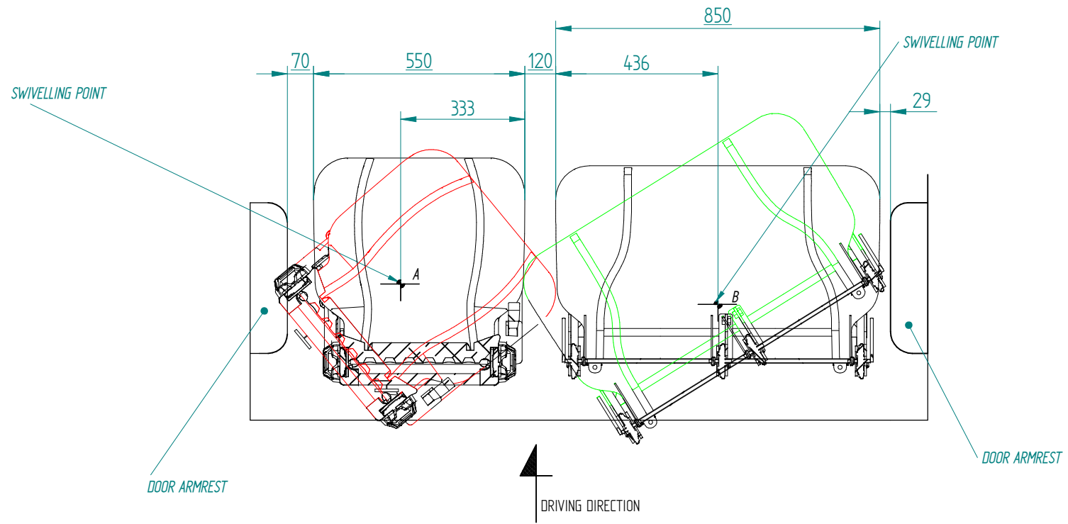
3-SEATS SYSTEM FOR THE CAB OF DUCATO X250-VEHICLE (PEUGEOT - CITROEN)
